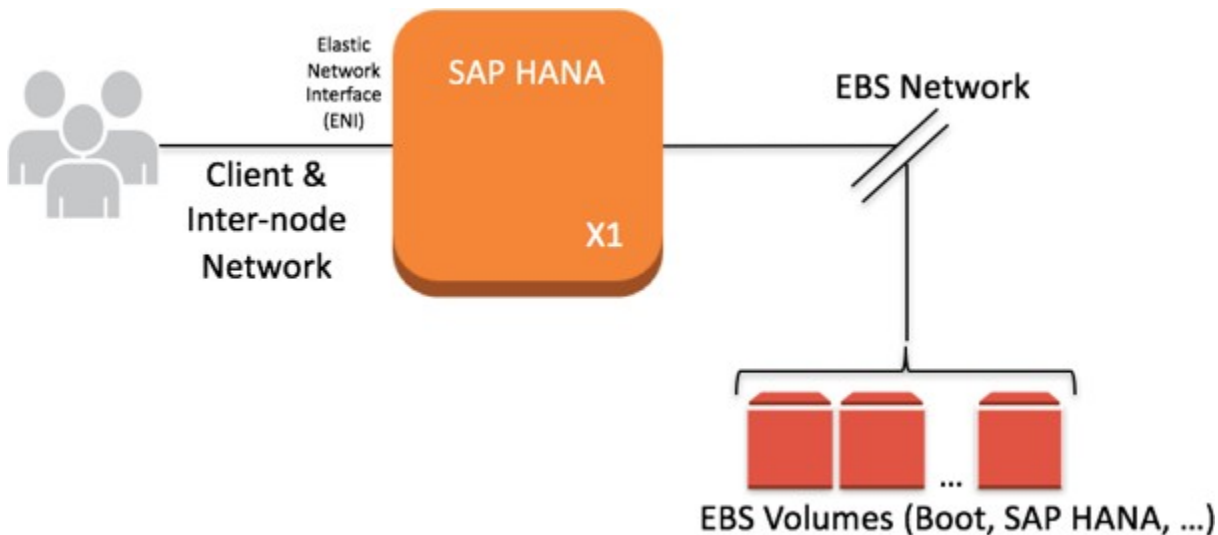
Figure 9: EBS-optimized instances
