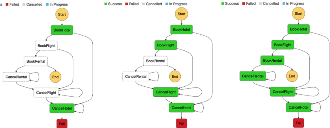
Figure 21: Step Functions state machine Saga pattern
