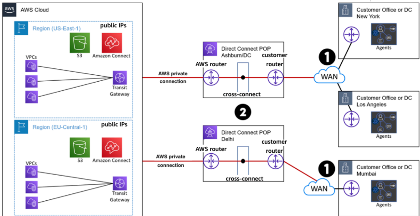
Reference architecture for a physical cross-connect to Direct Connect
