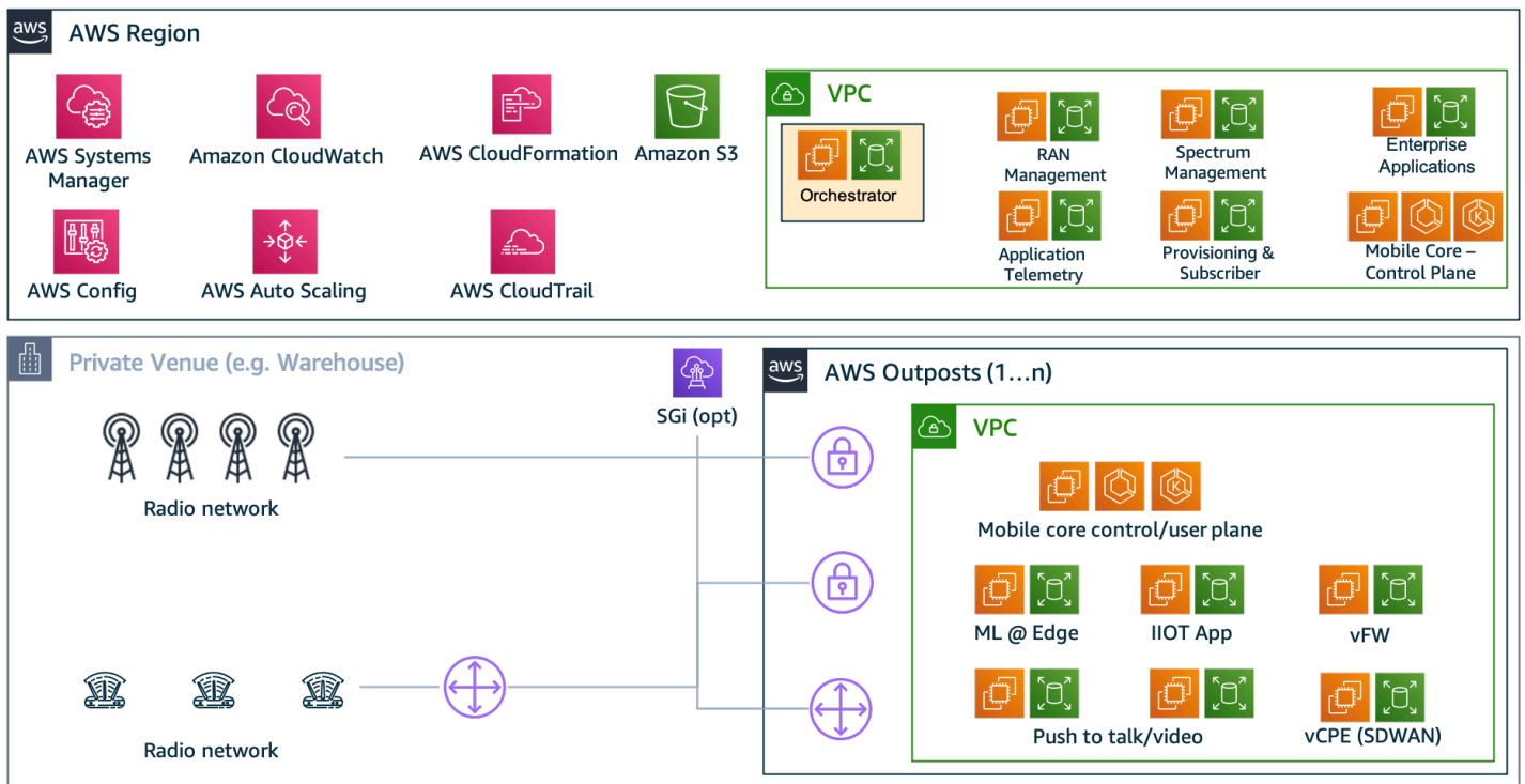
Figure 8 – Mobile private network operations and orchestration
