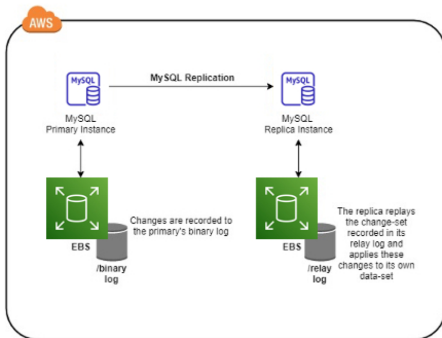
Binary log file position-based replication process
