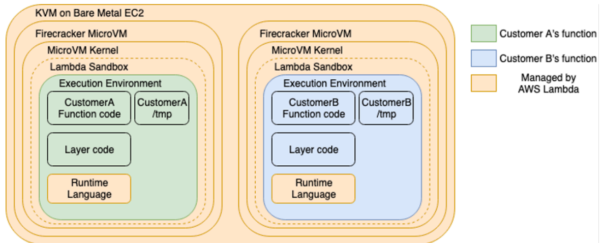
Isolation model for AWS Lambda Workers
