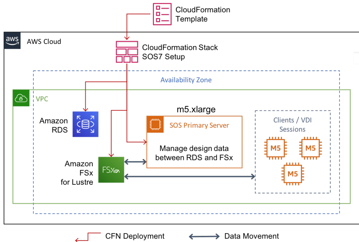
AWS Managed Services reference architecture example
