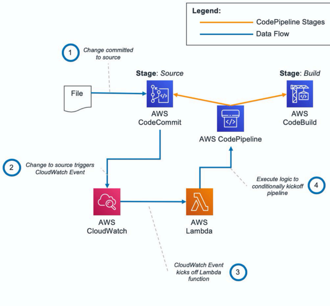
Architecture pattern for kicking off pipeline based on custom logic
