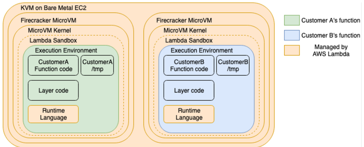
Figure 3 – Isolation model for AWS Lambda Workers
