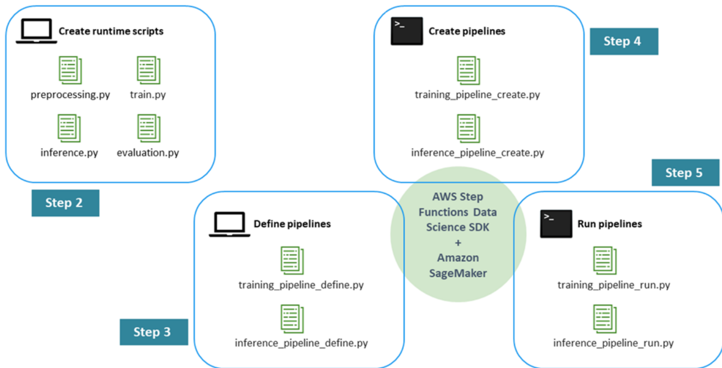
Steps for creating the training and inference pipeline
